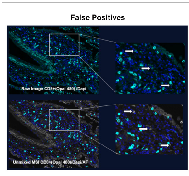
FIGURE 5. Arrows in the lung cancer raw image point to AF that is being incorrectly identified as CD8+. When AF is unmixed into its own channel (shown in the unmixed image as gray), we can visualize the difference.
